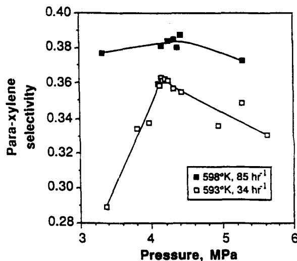
Figure 22. p -Xylene selectivity as a function of pressure at near-critical conditions (Collins et al., 1988).
