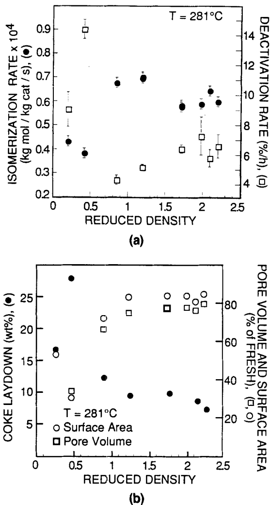
Figure 17. End-of-run results from 1-hexene isomerization at different sub- and supercritical densities (Ginosar and Subramaniam, 1994).
