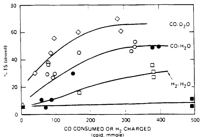
Figure 24. Coal conversion to toluene-solubles at 400°C for a 20-min reaction in different reaction environments.
