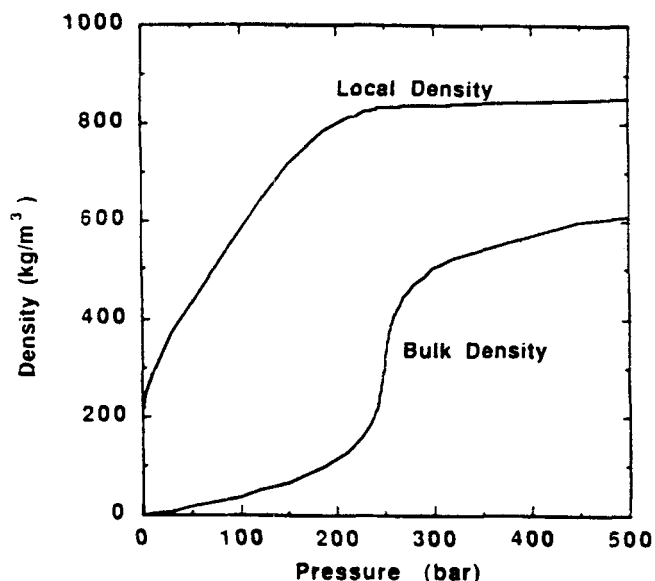
Figure 35. Local and bulk water density 2.2\text{ \AA} from the center of an ion at 385^{\circ}\text{C} (Flarsheim et al., 1989).
