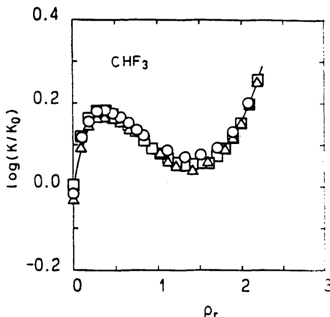
Figure 11. Equilibrium constant for 2-methyl-2-nitrosopropane dimerization in \text{CHF}_3 at 60.9^\circ\text{C} as a function of reduced density (Kimura and Yoshimura, 1992a).
