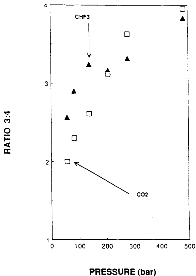
Figure 4. Effect of pressure on selectivity.
