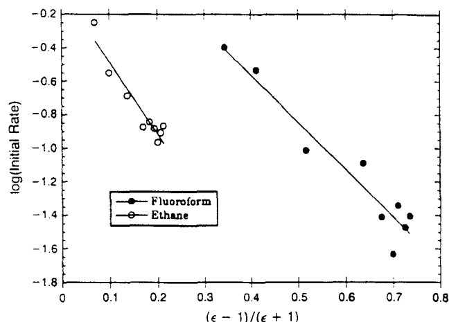
Figure 21. Kirkwood plot for lipase-catalyzed reaction in SC fluoroform (●) and SC ethane (○) (Kamat et al., 1993).
