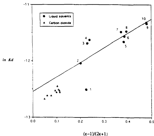
Figure 42. Kirkwood correlation for decomposition of azobis(isobutyronitrile) at 59.4°C in liquid solvents (●) and SC CO 2 (△) (Guan et al., 1993).
