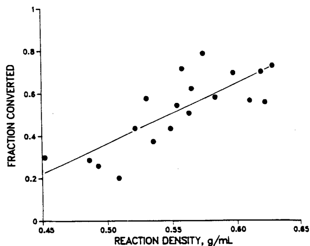
Figure 39. Effect of water density on conversion of 0.01 mole fraction 1,3-butanediol solution at 425°C for 30 min (West and Gray, 1987).
