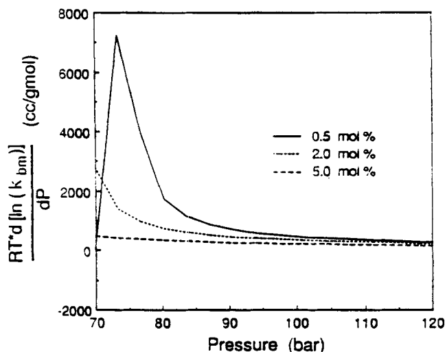
Figure 8. Effect of pressure predicted for the rate constant for benzophenone triplet plus isopropanol in SC \text{CO}_2 at different alcohol concentrations (Chateaufneuf et al., 1992).
