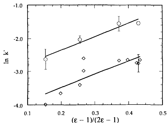
Figure 32. Kirkwood plot for oxidation kinetics in SC water at 380°C.
