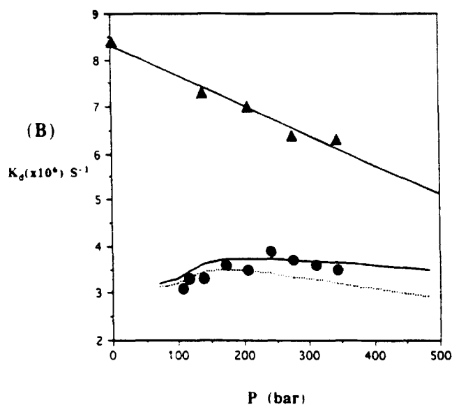
Figure 43. Rate constant for decomposition of azobis(isobutyronitrile) at 59.4°C and different pressures.
