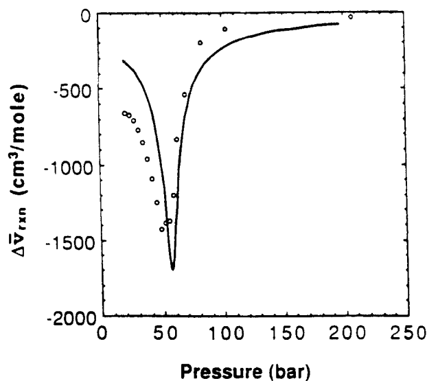
Figure 13. \Delta \bar{v}_{rxn} for tautomerization of 2-hydroxypyridine/2-pyridone in SC 1,1-difluoroethane at 403 K (Peck et al., 1989).
