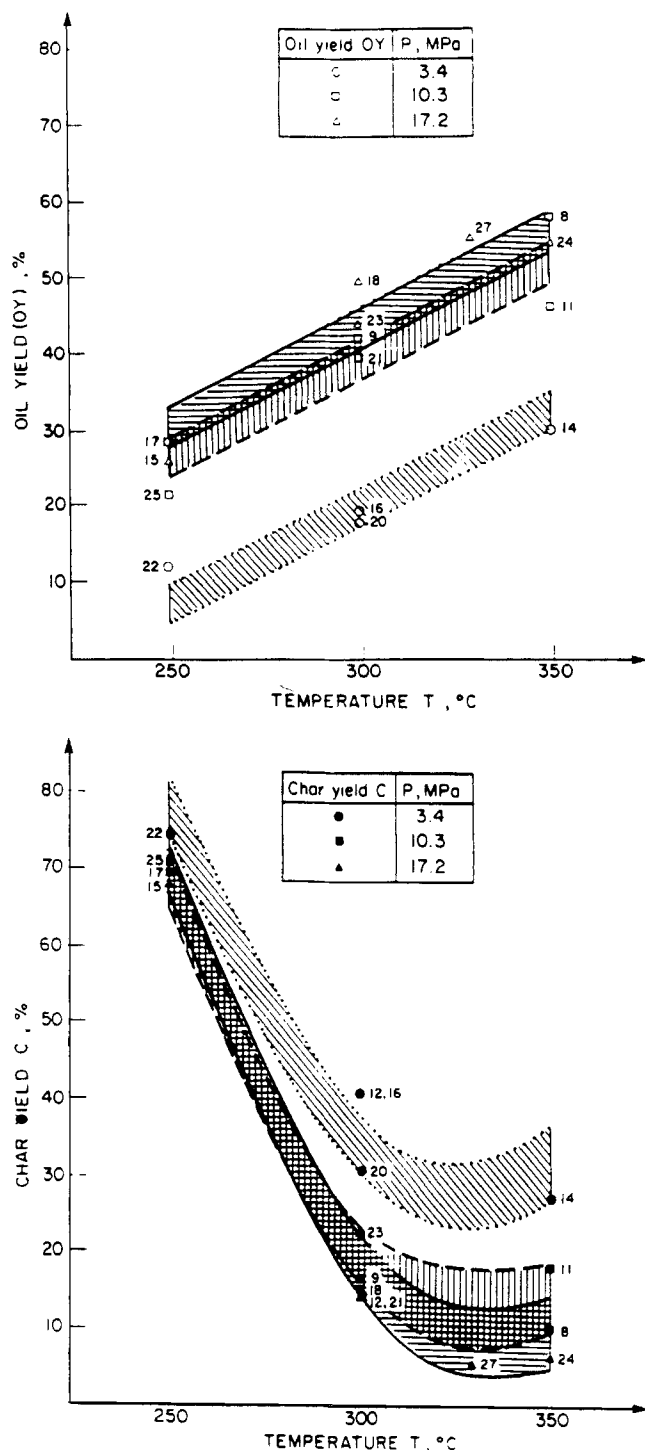
Figure 37. Effect of temperature and pressure on oil and char yield from wood liquefaction in methanol (Poirer et al., 1987).
