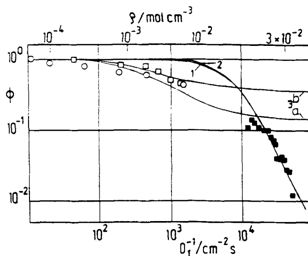
Figure 6. Quantum yields for I 2 photolysis in CO 2 as a function of reciprocal diffusivity and density.
