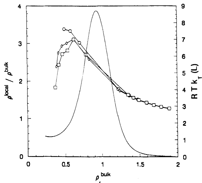
Figure 7. Local density enhancement about di-tert-butyl nitroxide radicals (discrete points correspond to different concentrations) and isothermal compressibility (smooth curve) as a function of reduced bulk density for SC ethane at 308 K (Carlier and Randolph, 1993).
