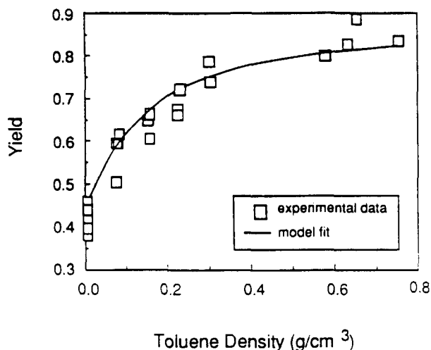
Figure 27. Effect of SC toluene density on benzyl phenyl ether yield at 320°C (yield = 1-conversion) (Wu et al., 1991b).
