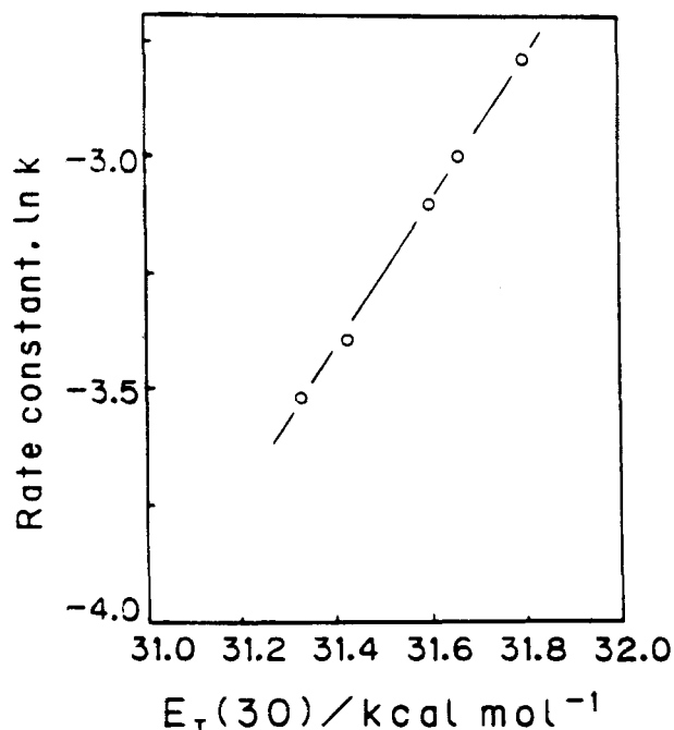
Figure 14. Rate constant for cycloaddition of isoprene and methyl acrylate in SC CO 2 at 323 K correlated with E_T(30) (Ikushima et al., 1992).
