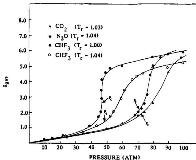
Figure 41. Solubility parameter as a function of pressure for different fluids near their critical temperature (Scholsky, 1993).
