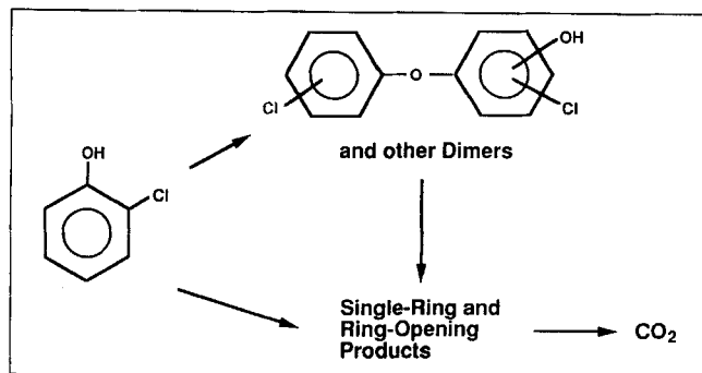
Figure 30. Global reaction network for 2-chlorophenol oxidation in SC water (Li et al., 1993).
