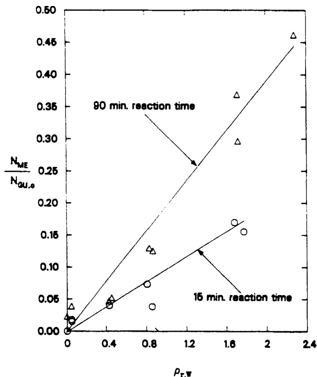
Figure 38. Effect of water density on methanol yield from guaiacol pyrolysis in water at 383°C (Lawson and Klein, 1985).
