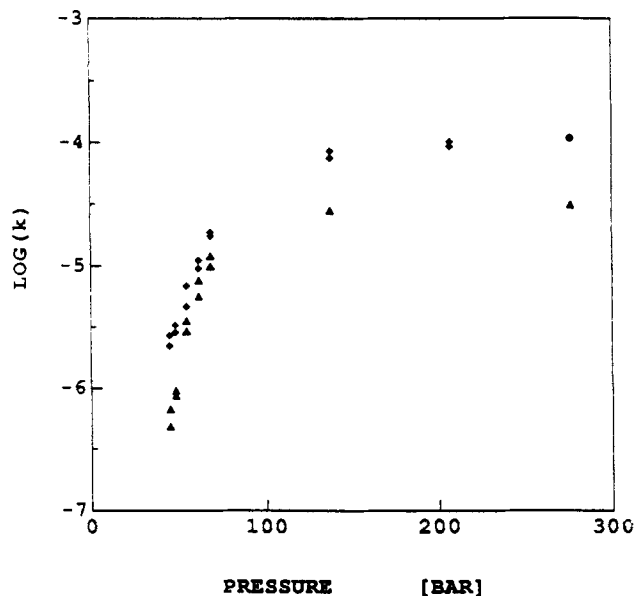
Figure 2. Effect of pressure on unimolecular reaction rate constant.
