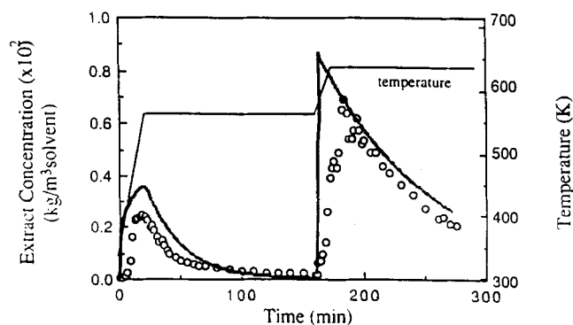
Figure 23. Comparison of model calculations and experimental data (open circles) for temperature-programmed coal extraction in SC t -butanol (Zhang et al., 1993).
