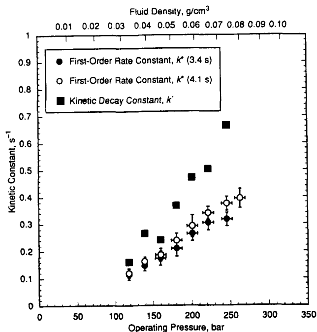
Figure 31. Effect of pressure (and water density) on CO oxidation kinetics in SC water at 570°C (Holgate and Tester, 1994a).
