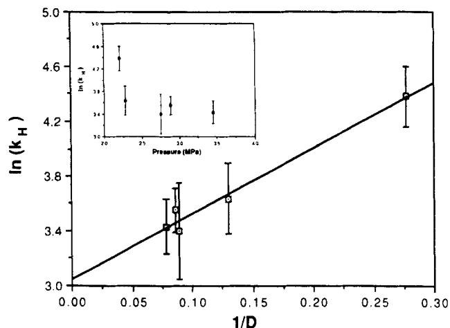
Figure 40. Effect of pressure and dielectric constant (D) on acid-catalyzed hydrolysis rate constant at 375°C (Narayan and Antal, 1990).
