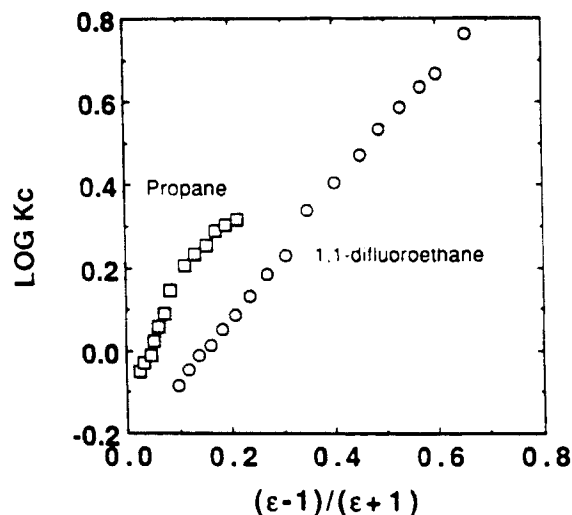
Figure 12. Kirkwood plot for equilibrium constant for tautomerization of 2-hydroxypyridine/2-pyridone in SC propane at 393 K and SC 1,1-difluoroethane at 403 K (Peck et al., 1989).
