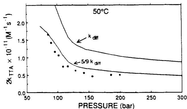
Figure 9. Rate constant for diffusion-controlled bimolecular reaction (triplet-triplet annihilation of benzophenone) in SC CO 2 at 50°C.
