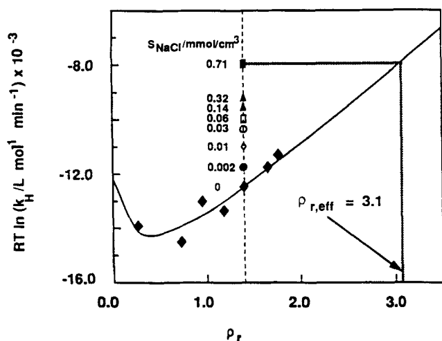
Figure 26. Effect of added salts and water density on guaiacol hydrolysis kinetics (Klein et al., 1990).
