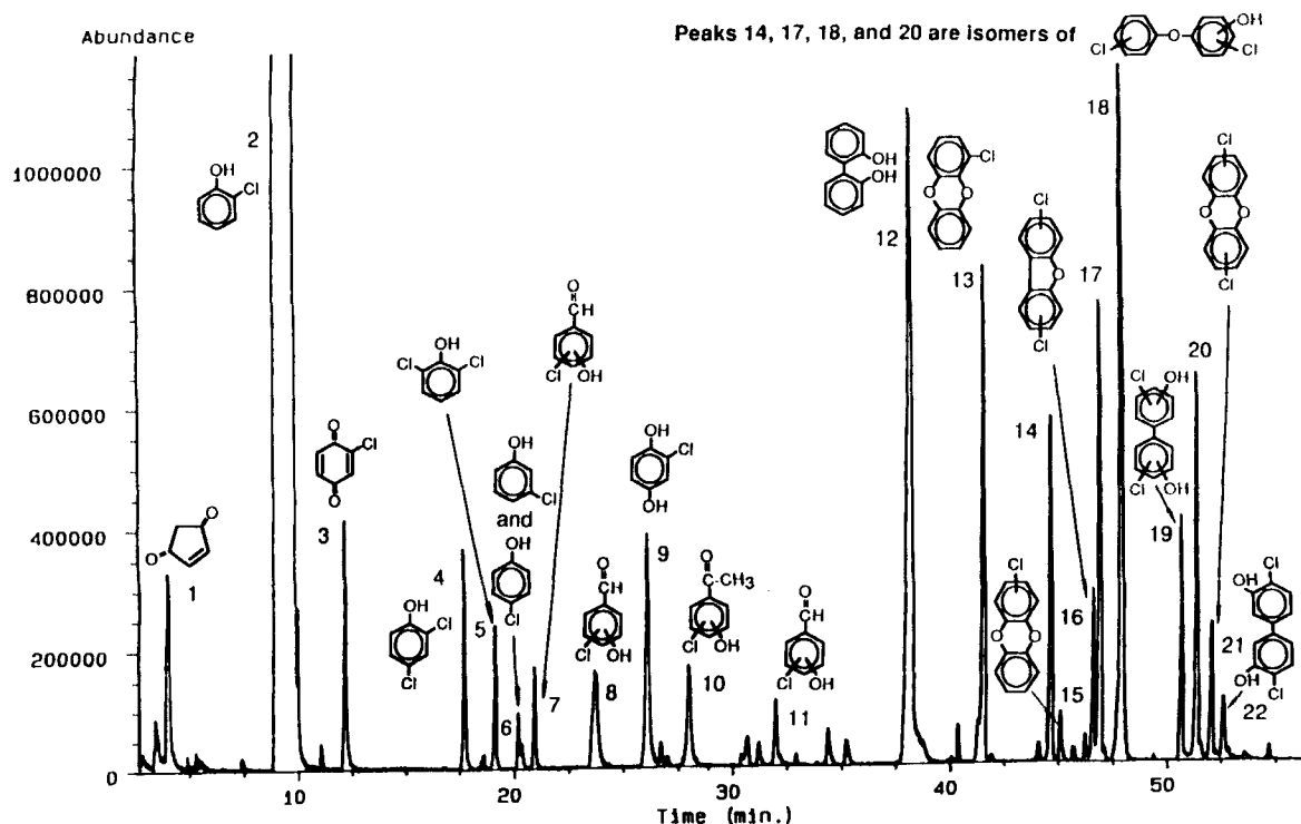
Figure 29. Total ion chromatogram of 2-chlorophenol oxidation products in SC water at 380°C, 278 atm and 24.7 s residence time (Li et al., 1993).
