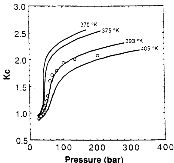
Figure 5. Effect of pressure on equilibrium constant.
