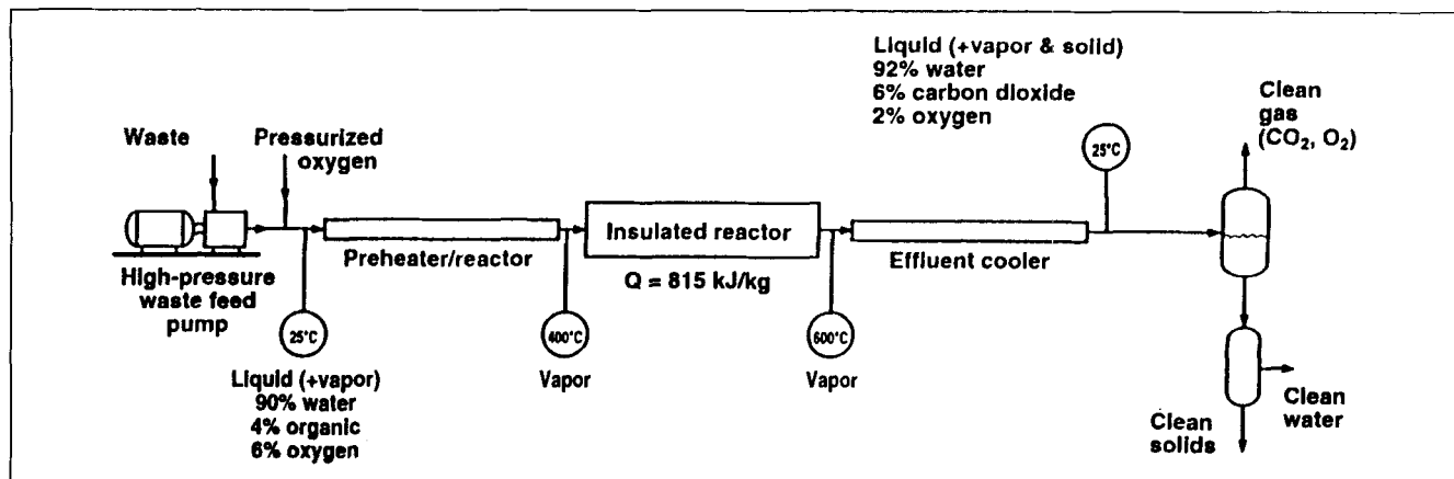
Figure 28. Simplified flowsheet for a SCWO process with representative compositions and temperatures (Modell et al., 1992).
