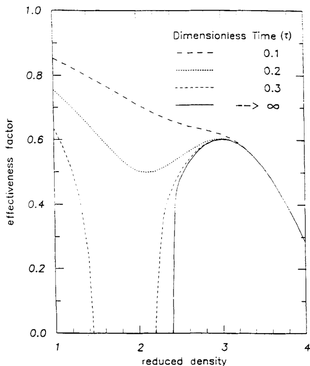
Figure 16. Effectiveness factor map for 1-hexene isomerization at SC conditions (Baptist-Nguyen and Subramaniam, 1992).
