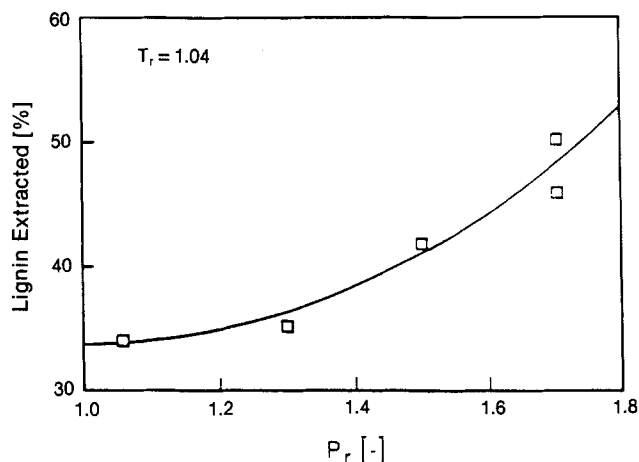
Figure 36. Effect of reduced pressure on lignin extraction by SC tert butyl alcohol (Goto et al., 1990a).
