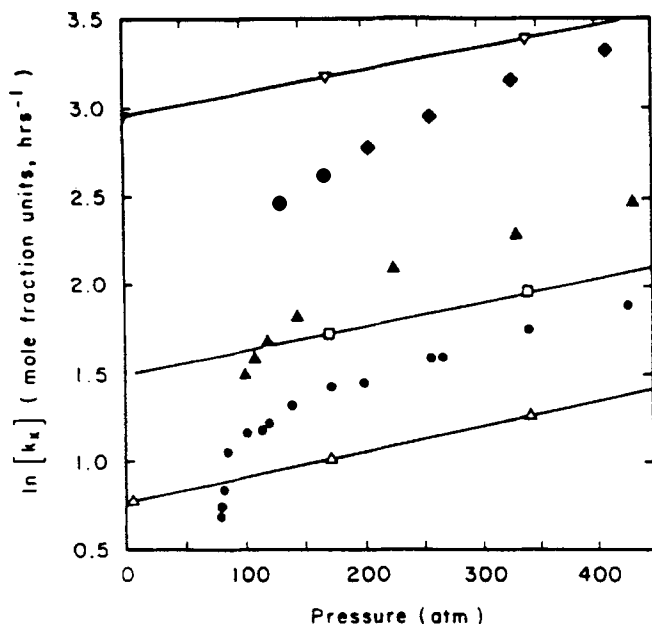
Figure 3. Effect of pressure on bimolecular reaction rate constant.
