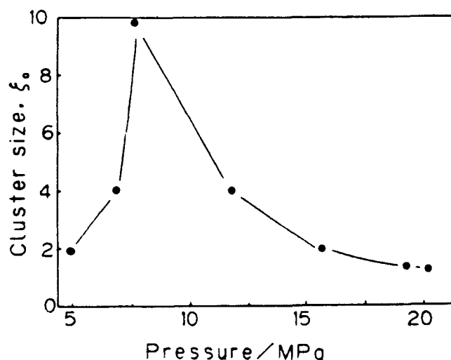
Figure 15. Cluster size for cycloaddition of isoprene and methyl acrylate in SC CO 2 at 323 K (Ikushima et al., 1992).
