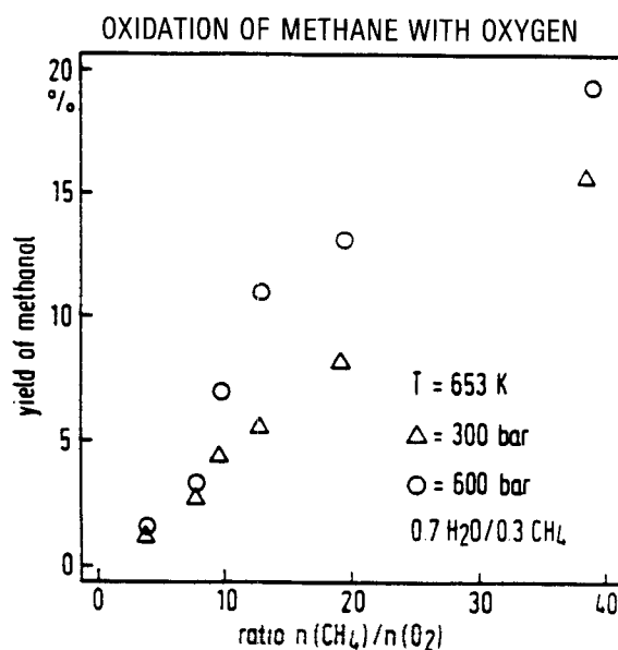
Figure 34. Fraction of methane reacted that forms methanol during partial oxidation in SC water at 653 K (Franck, 1991a).
