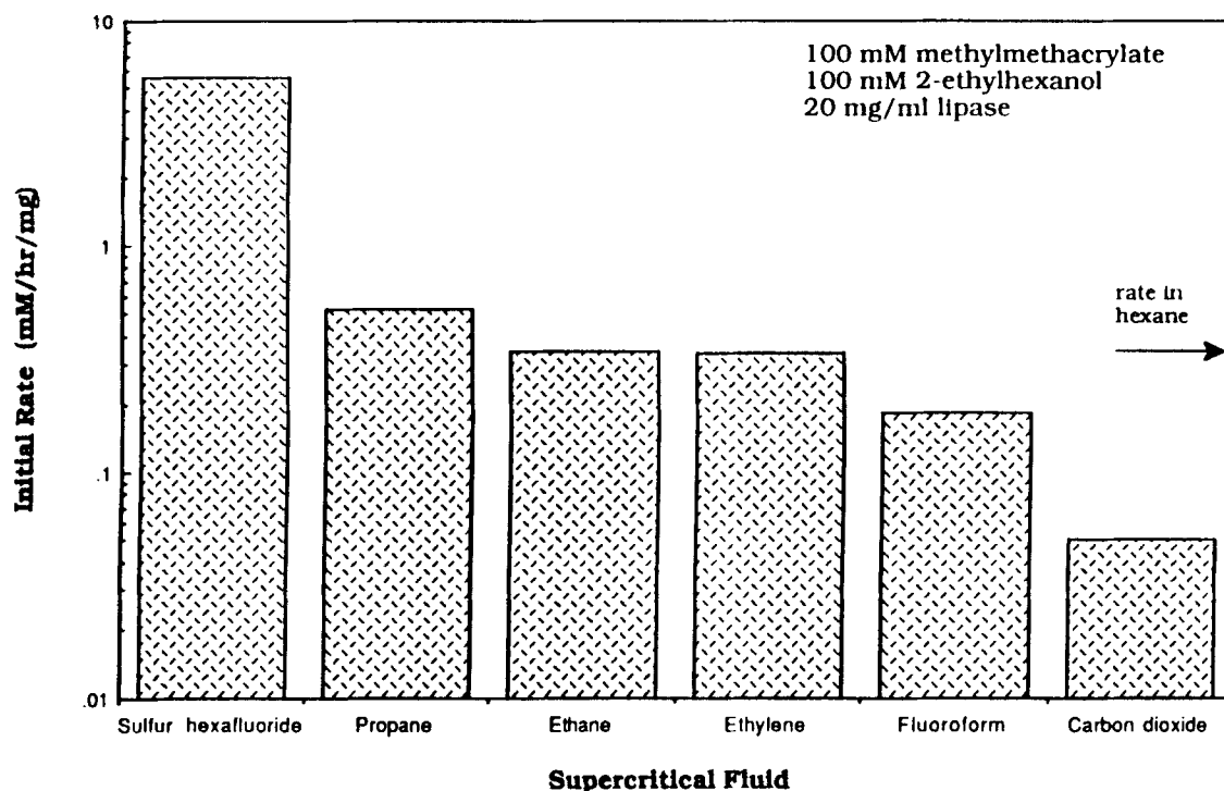
Figure 20. Rates of lipase-catalyzed reaction between 2-ethylhexanol and methylmethacrylate in SCFs at 1,600 psi (11 MPa) and 45°C (Kamat et al., 1992).
