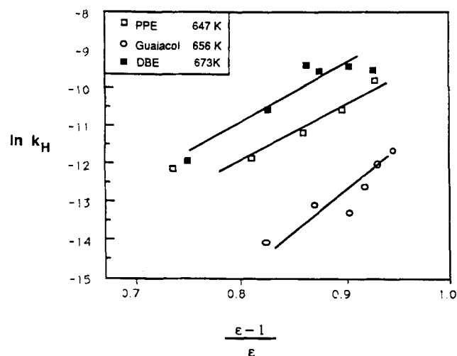
Figure 25. Kirkwood plot for the hydrolysis rate constant for phenethyl phenyl ether (PPE), guaiacol, and dibenzyl ether (DBE) in SC water (Klein et al., 1990).
