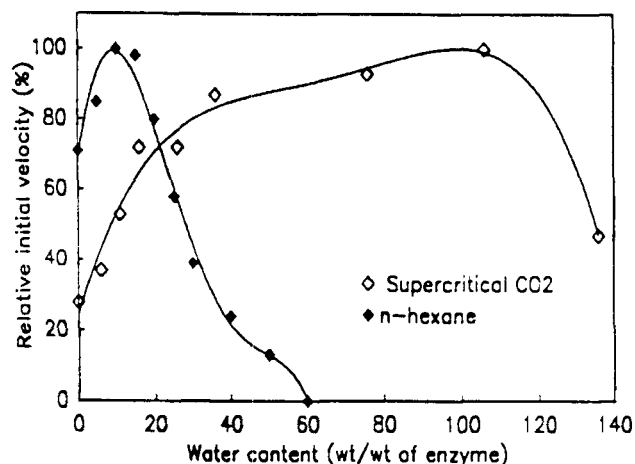
Figure 18. Effect of water content of fluid phase on enzyme-catalyzed reaction rate in SC CO 2 and n -hexane at 40°C (Marty et al., 1990).
