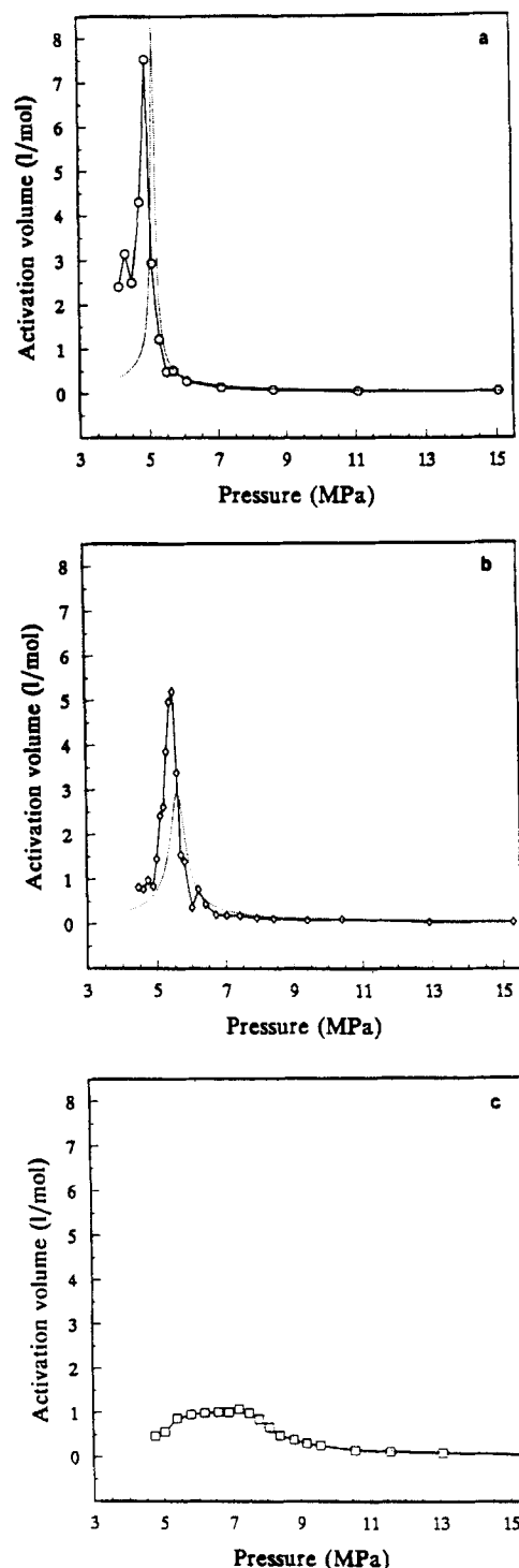
Figure 10. Activation volumes for diffusion-controlled reaction in SC ethane at 308, 313, and 331 K (Randolph and Carlier, 1992a).
