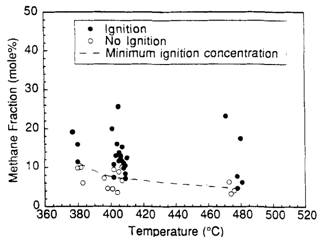
Figure 33. Explosive limits for methane in water (Steeper et al., 1992).
